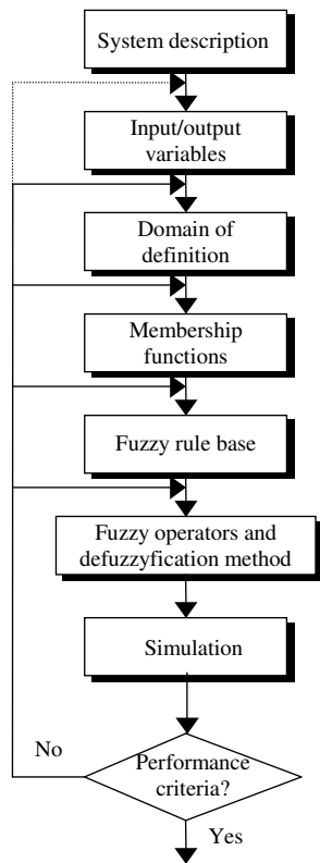
Fig. 3 Designing algorithm of a fuzzy controller
