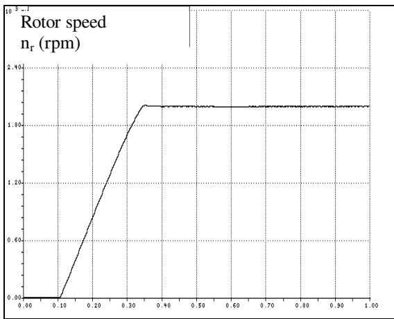
Fig. 8 Speed response
