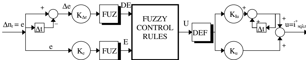
Fig. 2 Block diagram of the fuzzy-logic based speed controller
