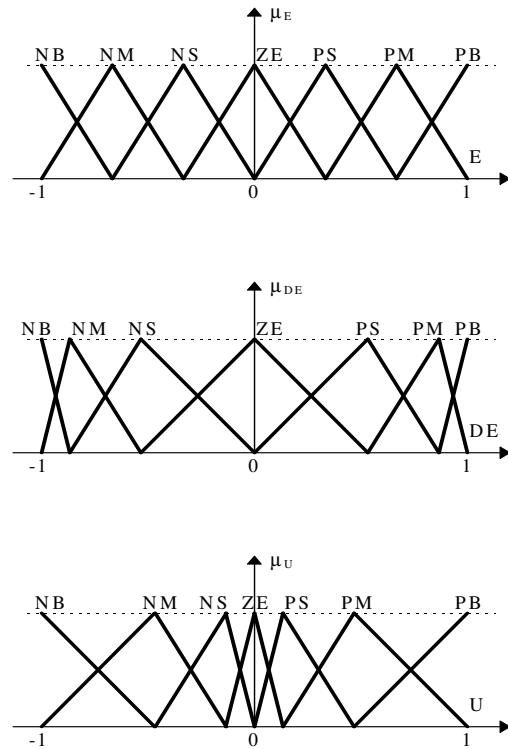
Fig. 4 Fuzzy membership functions (fuzzy numbers) of the linguistic variables E , DE and U
