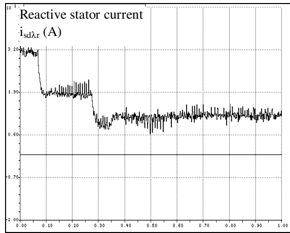
Fig. 11 Reactive component of stator current
