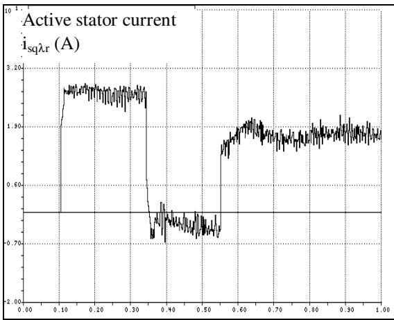
Fig. 10 Torque-producing component of the stator current
