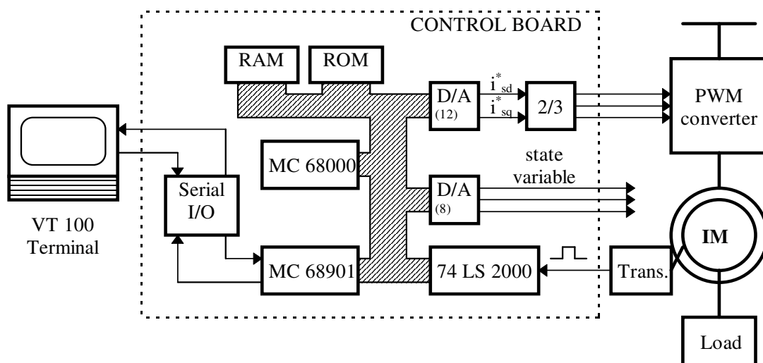
Fig. 7 Block diagram of the motion control board with MC68000
