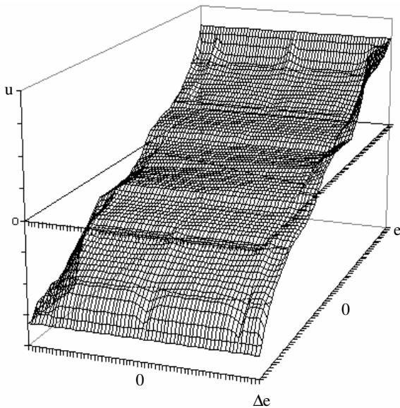
Fig. 6 Diagram u=f(e, \Delta e) of the fuzzy PID controller
