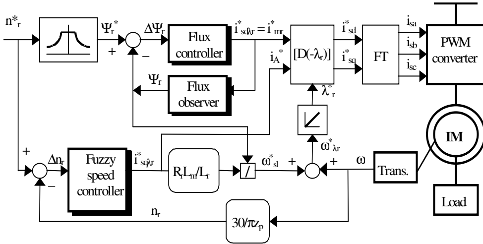
Fig. 1 Block-diagram of a speed control system with induction machine
