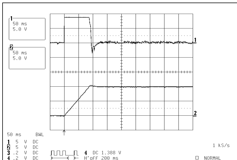
Fig. 12 Active component of the stator current (1) and speed (2) at a imposed value of 1500 rpm, by using a fuzzy speed controller
